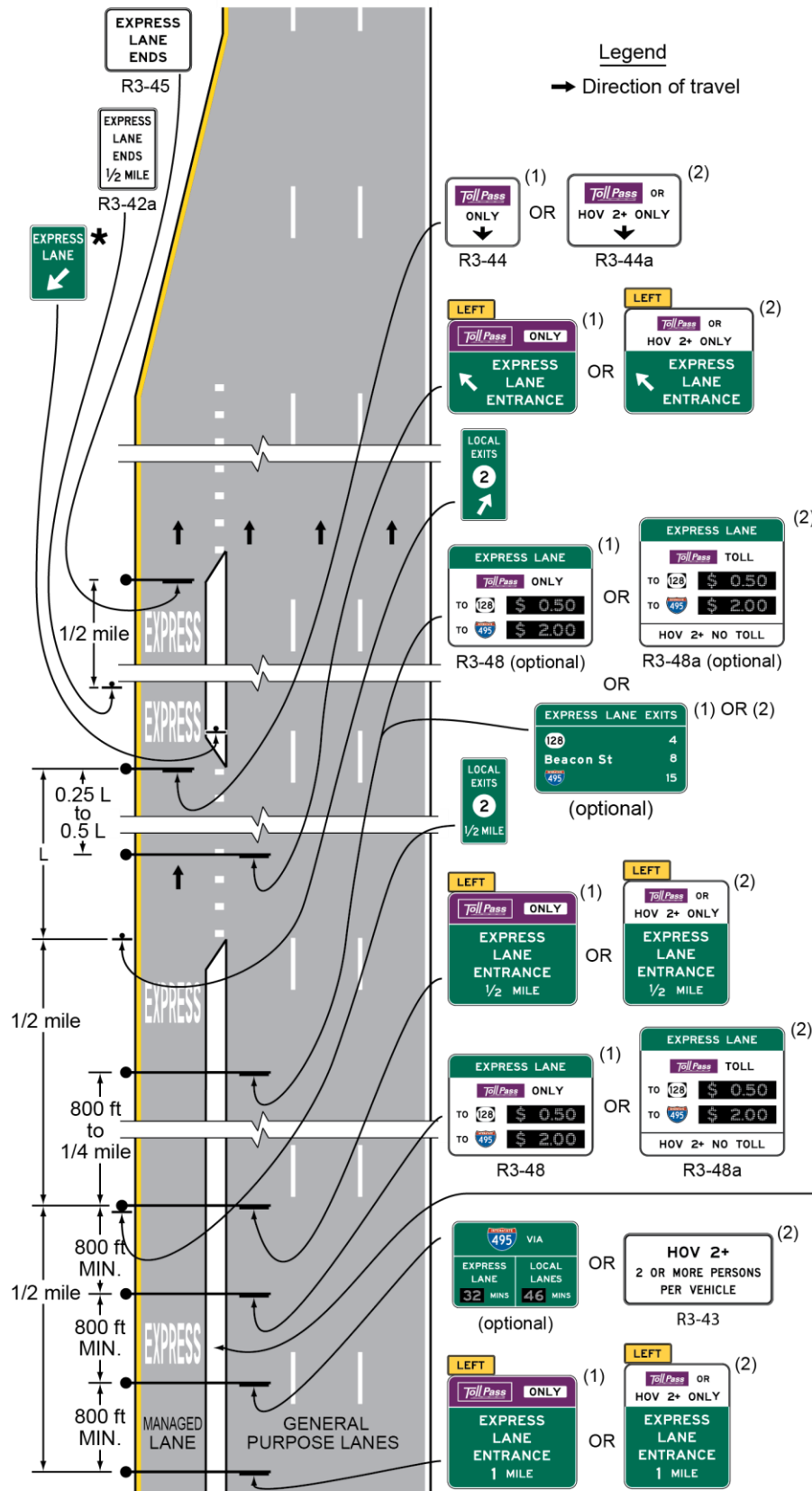
Figure 2G-24. Example of Signing for the Intermediate Entry to, Egress from, and End of Access-Restricted Priced Managed Lane
